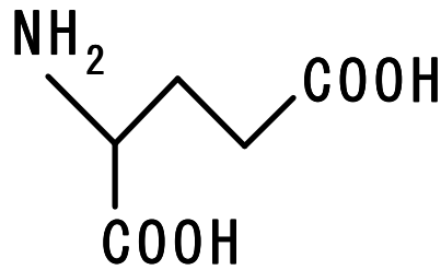
Glutamic acid
